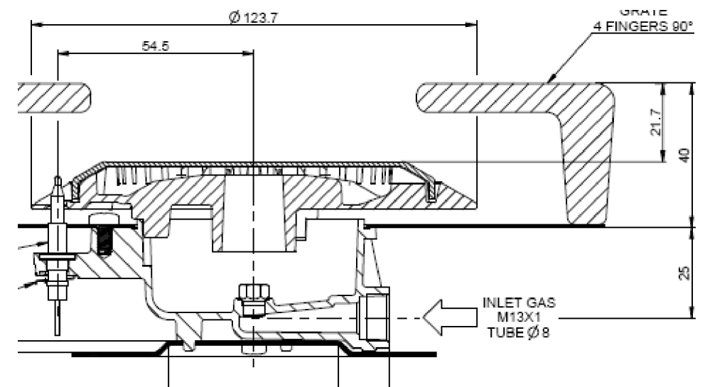
SECTION C-C
